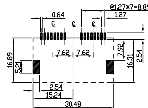
PC BOARD LAYOUT (COMPONENT SIDE OF BOARD)
